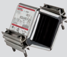
STRAUB-SQUARE-FLEX
