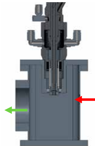
Step 1: Ionized air is blown into the loading head as soon as the screw arrives.
