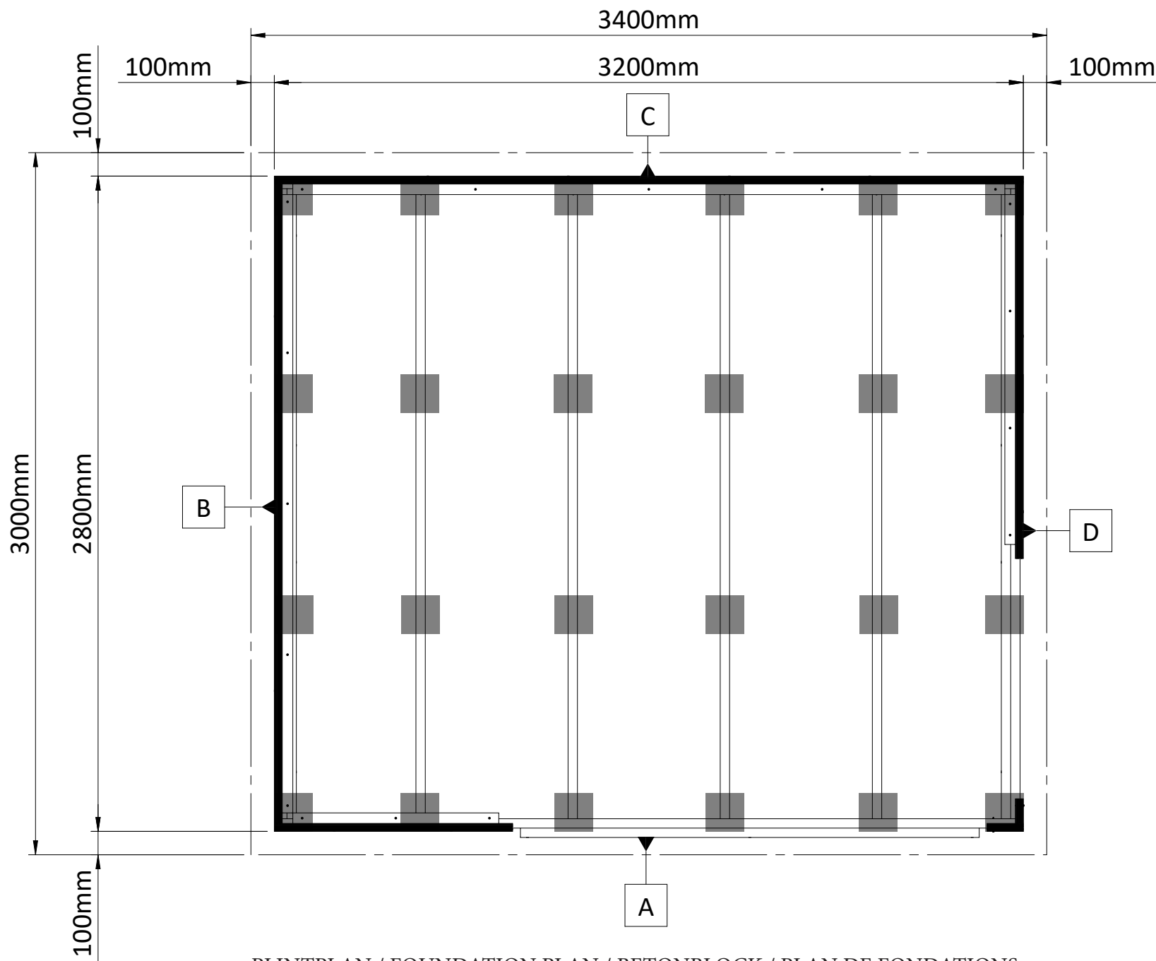
PLINTPLAN / FOUNDATION PLAN / BETONBLOCK / PLAN DE FONDATIONS
