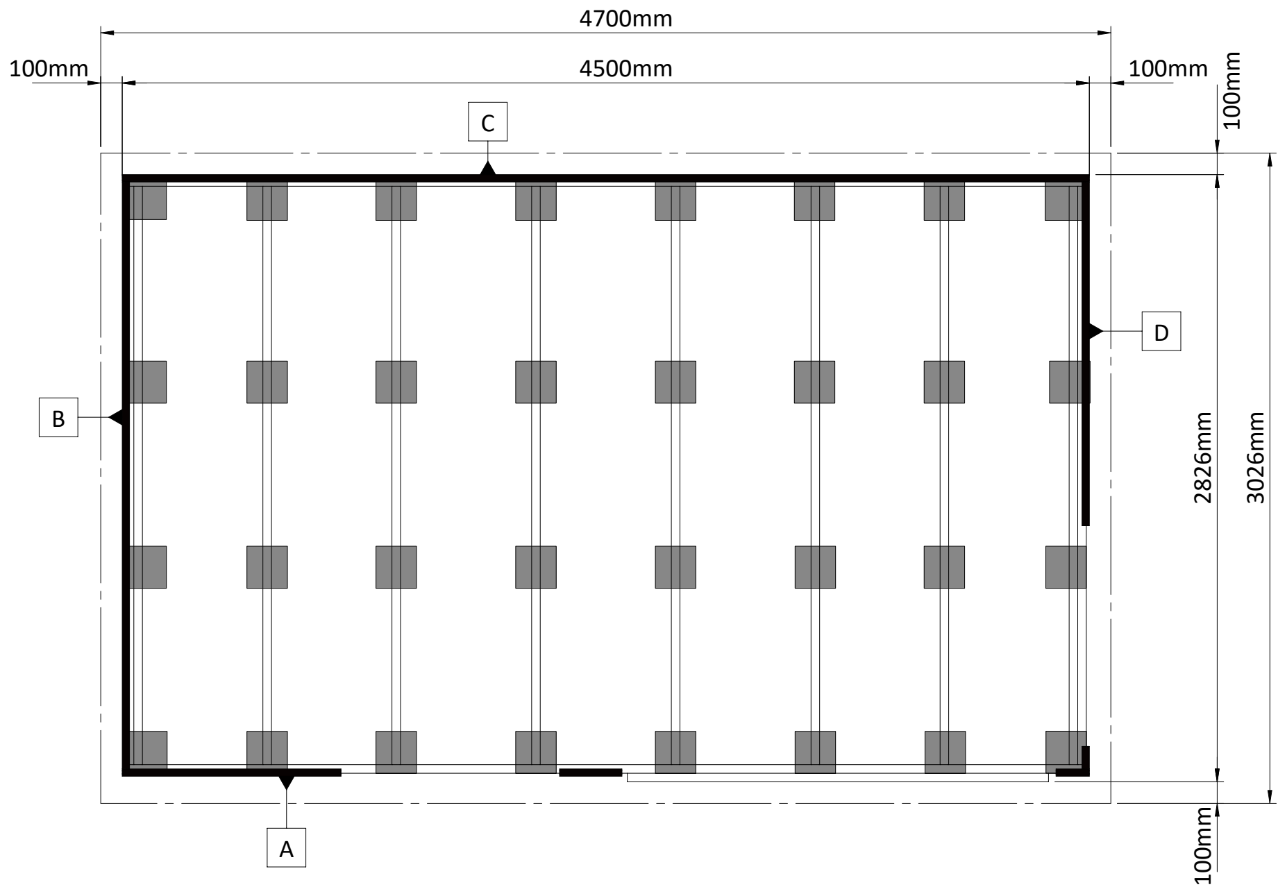
PLINTPLAN / FOUNDATION PLAN / BETONBLOCK / PLAN DE FONDATIONS
