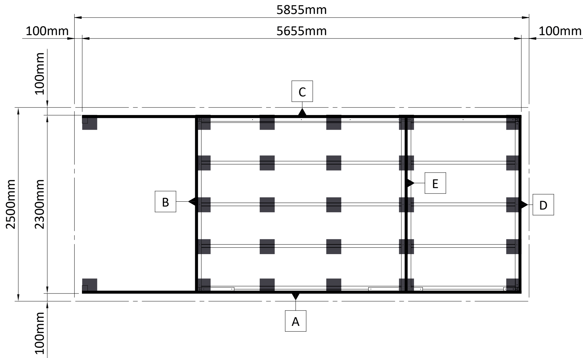
PLINTPLAN / FOUNDATION PLAN / BETONBLOCK / PLAN DE FONDATIONS
