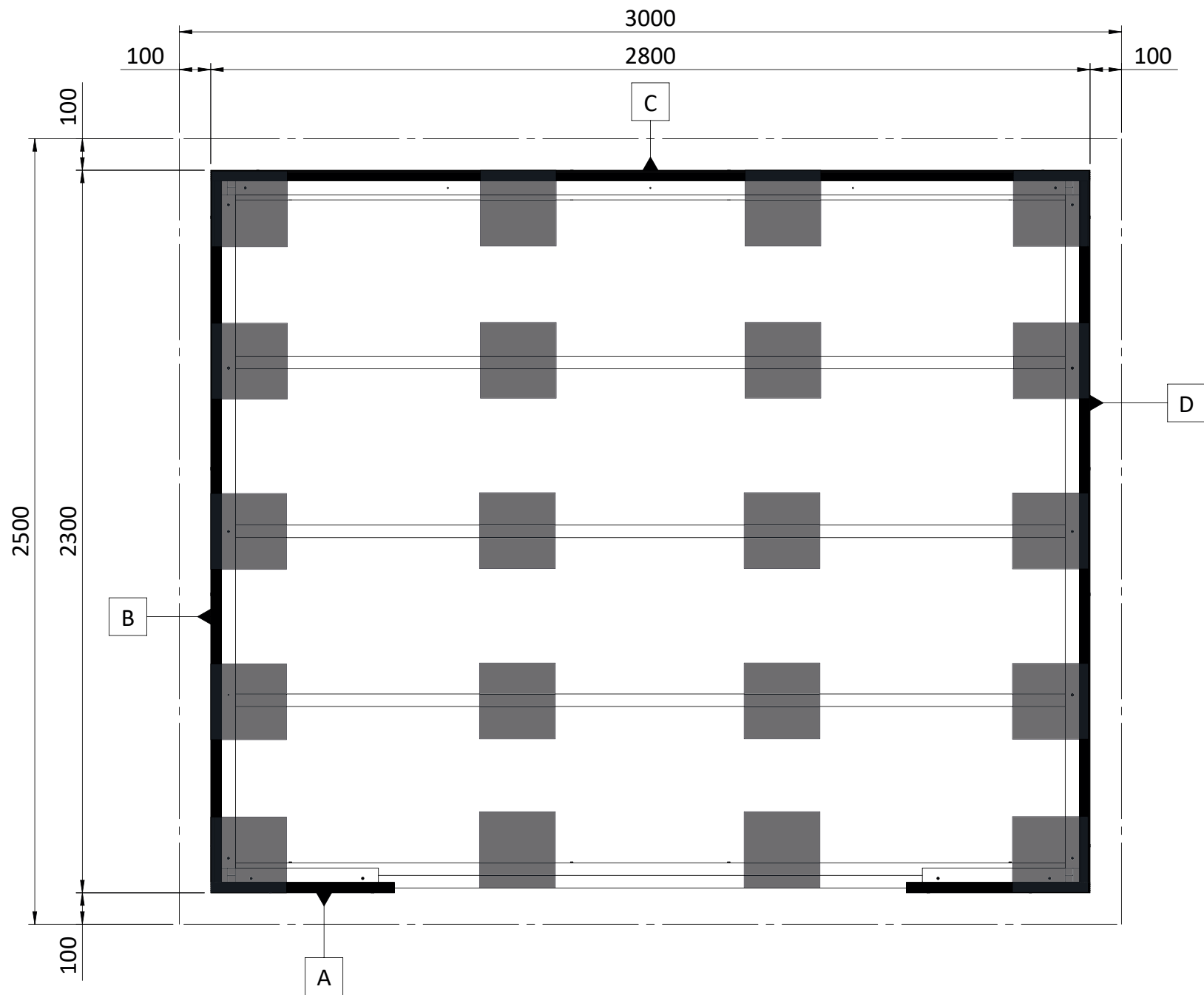
PLINTPLAN / FOUNDATION PLAN / BETONBLOCK / PLAN DE FONDATIONS
