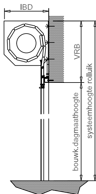
detail haakgoot
