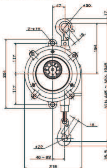
EWA-22/30
