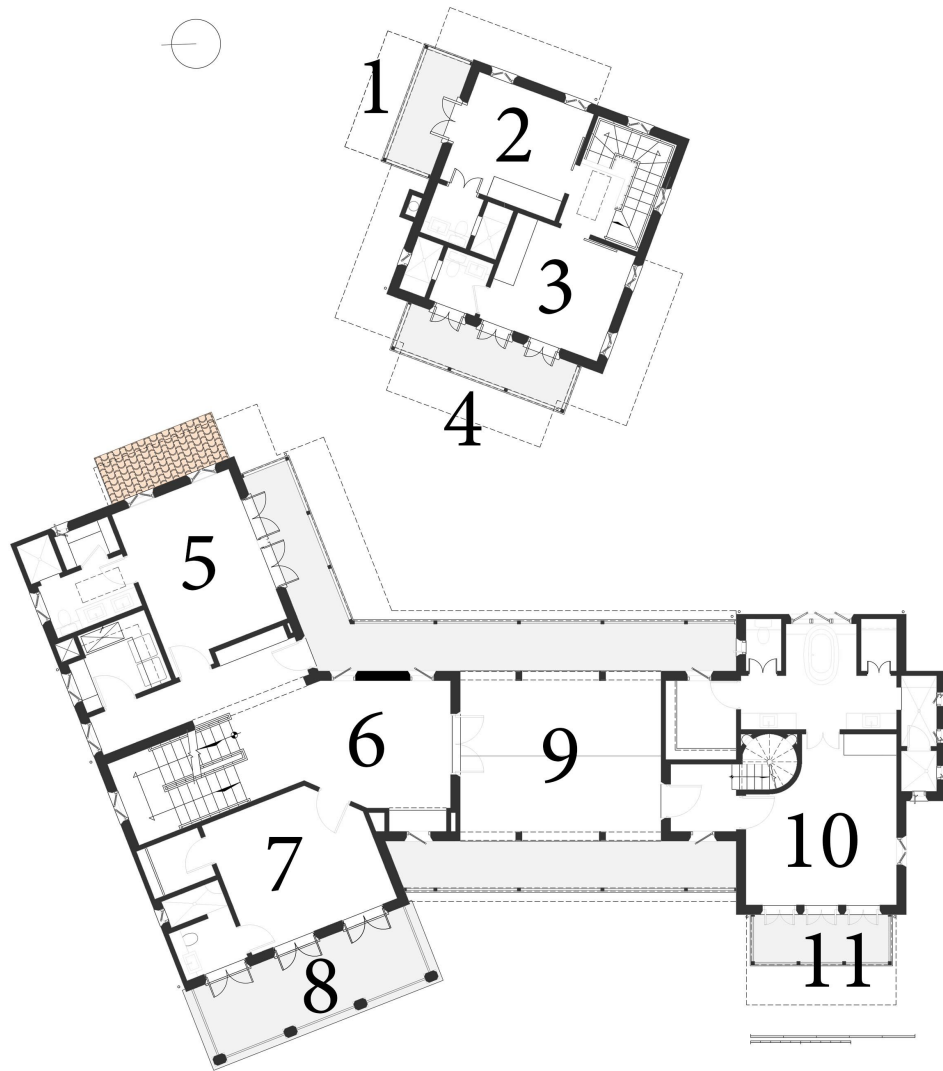
Second Level
