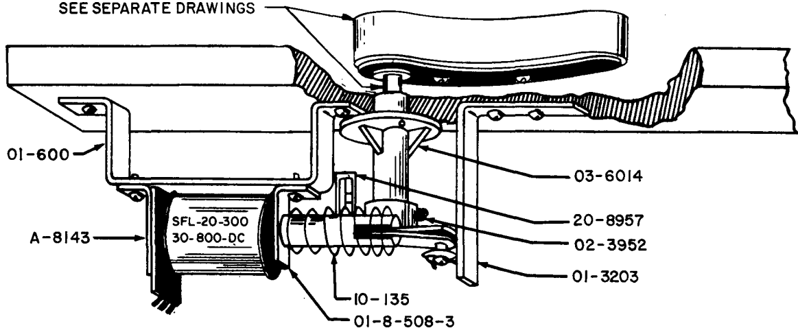
B-7060-2 CURVED FLIPPER ASSEMBLY COMPLETE B-7060-2L (LEFT) B-7060-2R (RIGHT)
