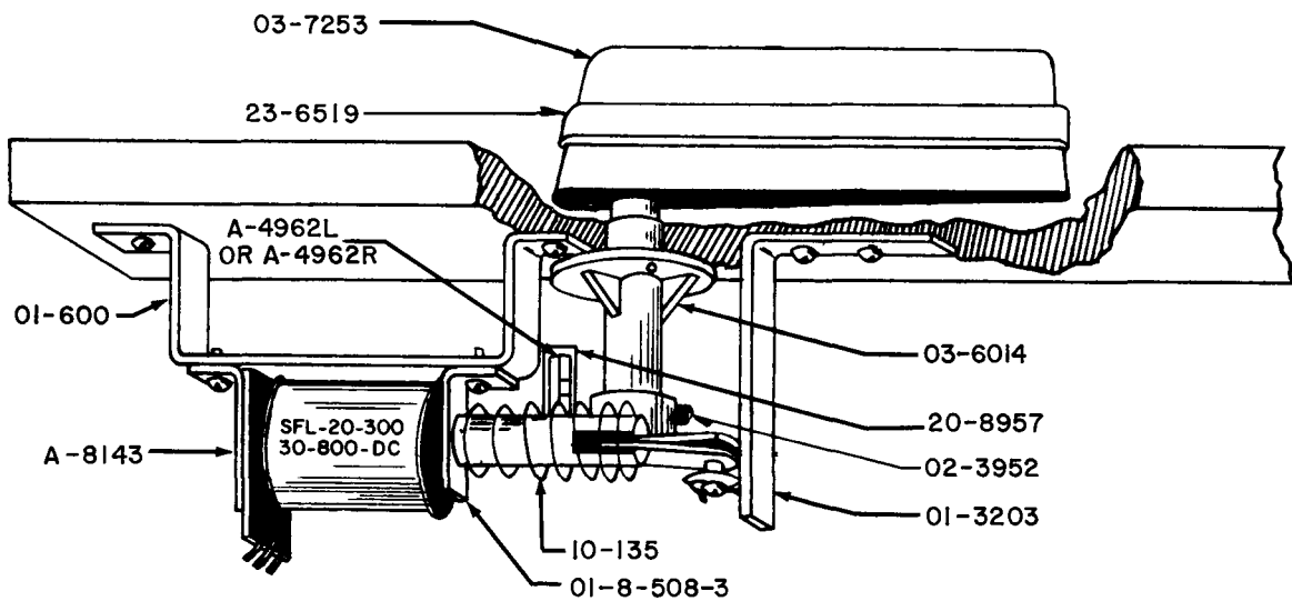
B-7060 STRAIGHT FLIPPER ASSEMBLY COMPLETE B-7060-L (LEFT) B-7060-R (RIGHT)
