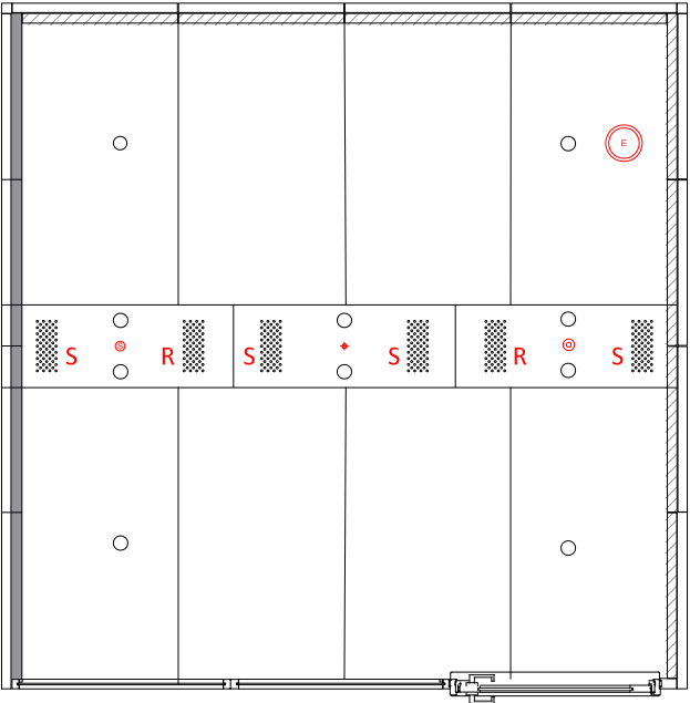
Ceiling Services
