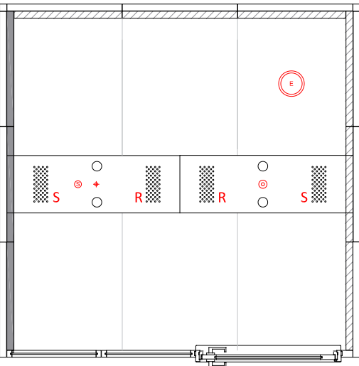
Ceiling Services
