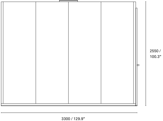
Side
