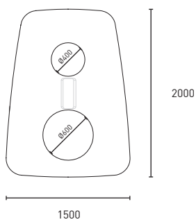
Ø400 + Ø600 Double Base, Lozenge Worktop
