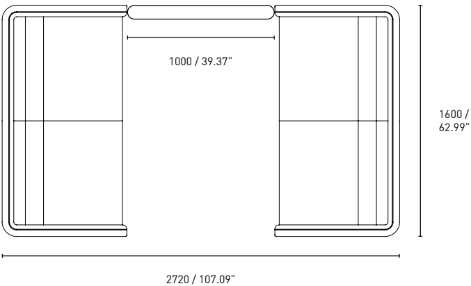
Four Seater Booth with 1000mm / 39.37" Panel
