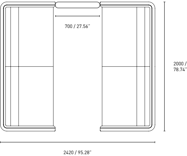
Six Seater Booth with 700mm / 27.56" Panel
