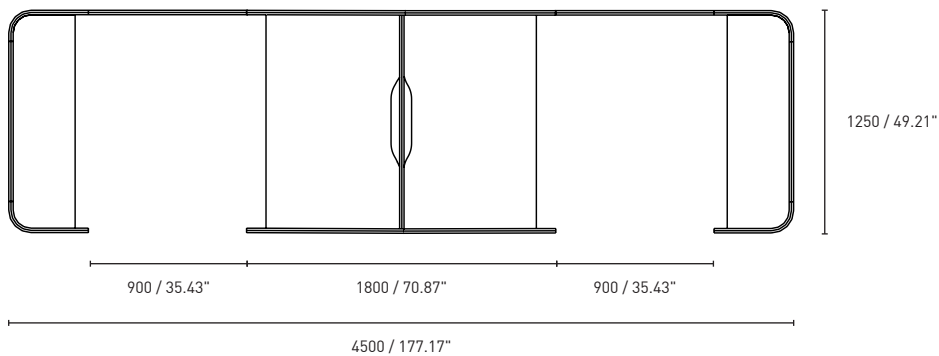
Enclosed Desk, Inward Facing, 2 Cluster with Ducted Side Panel
