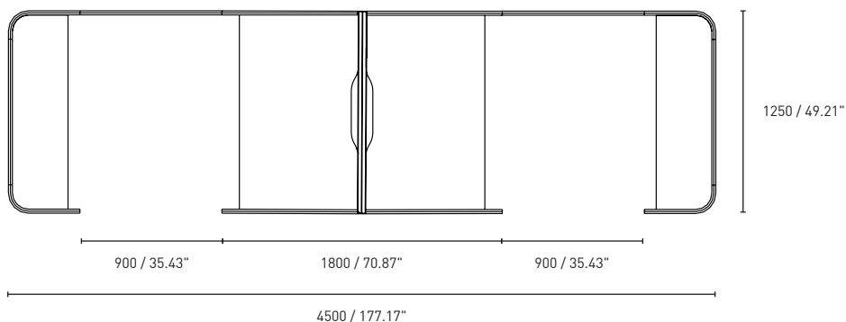
Enclosed Desk, Inward Facing, 2 Cluster with Ducted Middle Panel
