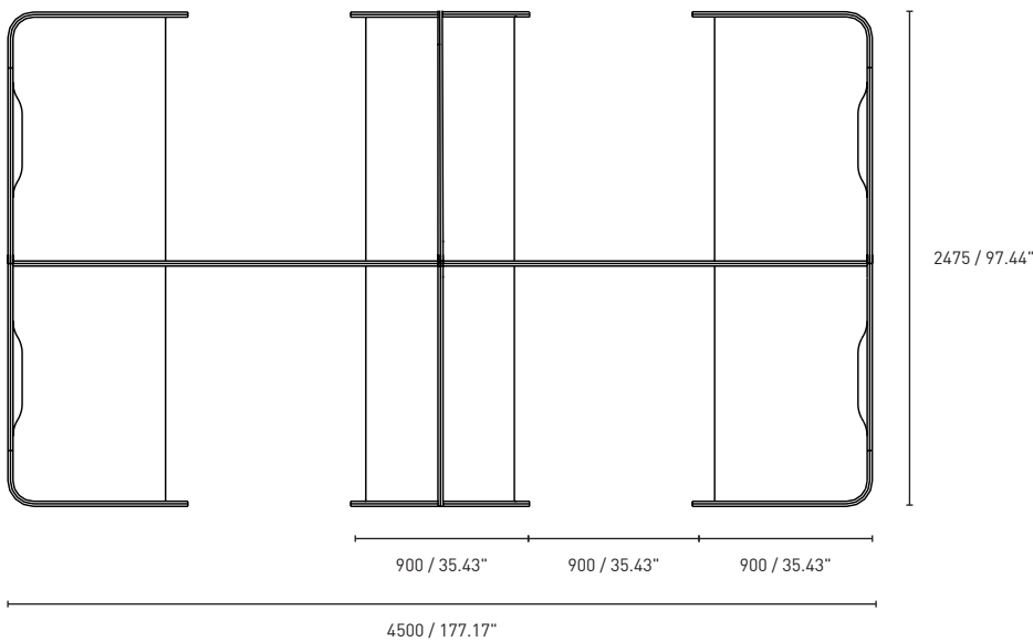
Enclosed, Side by Side, 4 Cluster, Ducted Middle Panel
