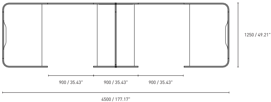
Enclosed Desk, Outward Facing, 2 Cluster
