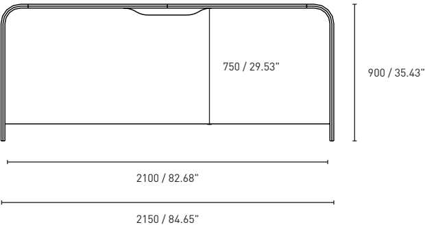
Two Person Desk
