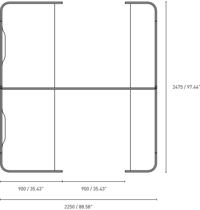
Enclosed, Side by Side
