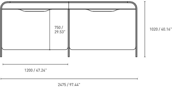
Two Person Side by Side Desk, Ducted Wall, Two Cluster
