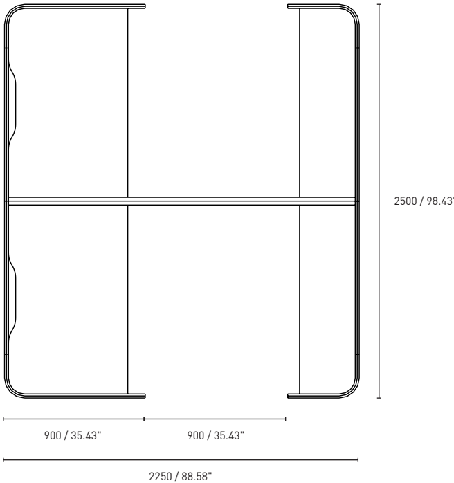
Enclosed, Side by Side, Ducted Middle Panel
