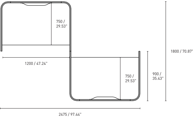
Opposite Facing Desk
