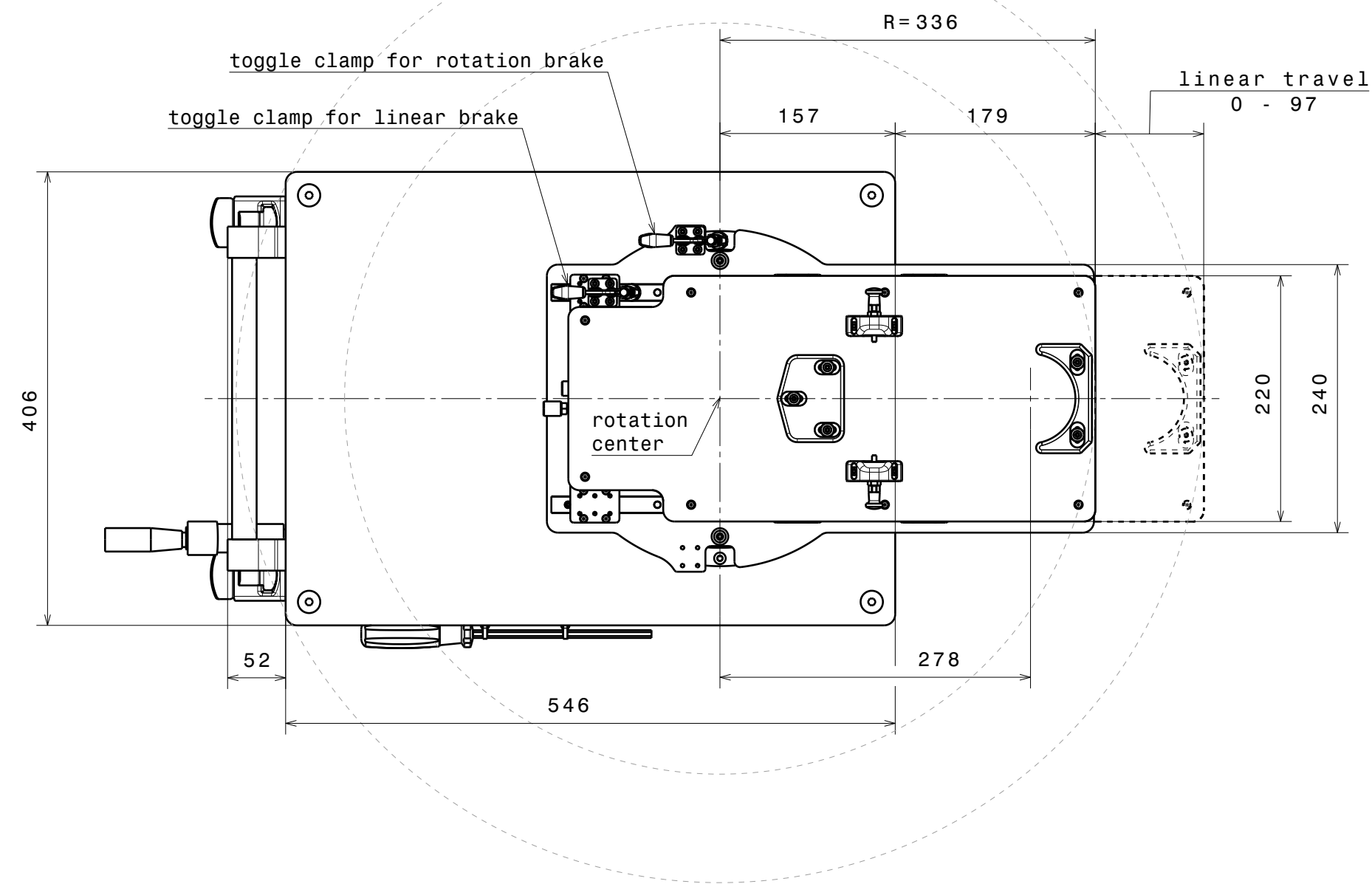
Tranpost Position
