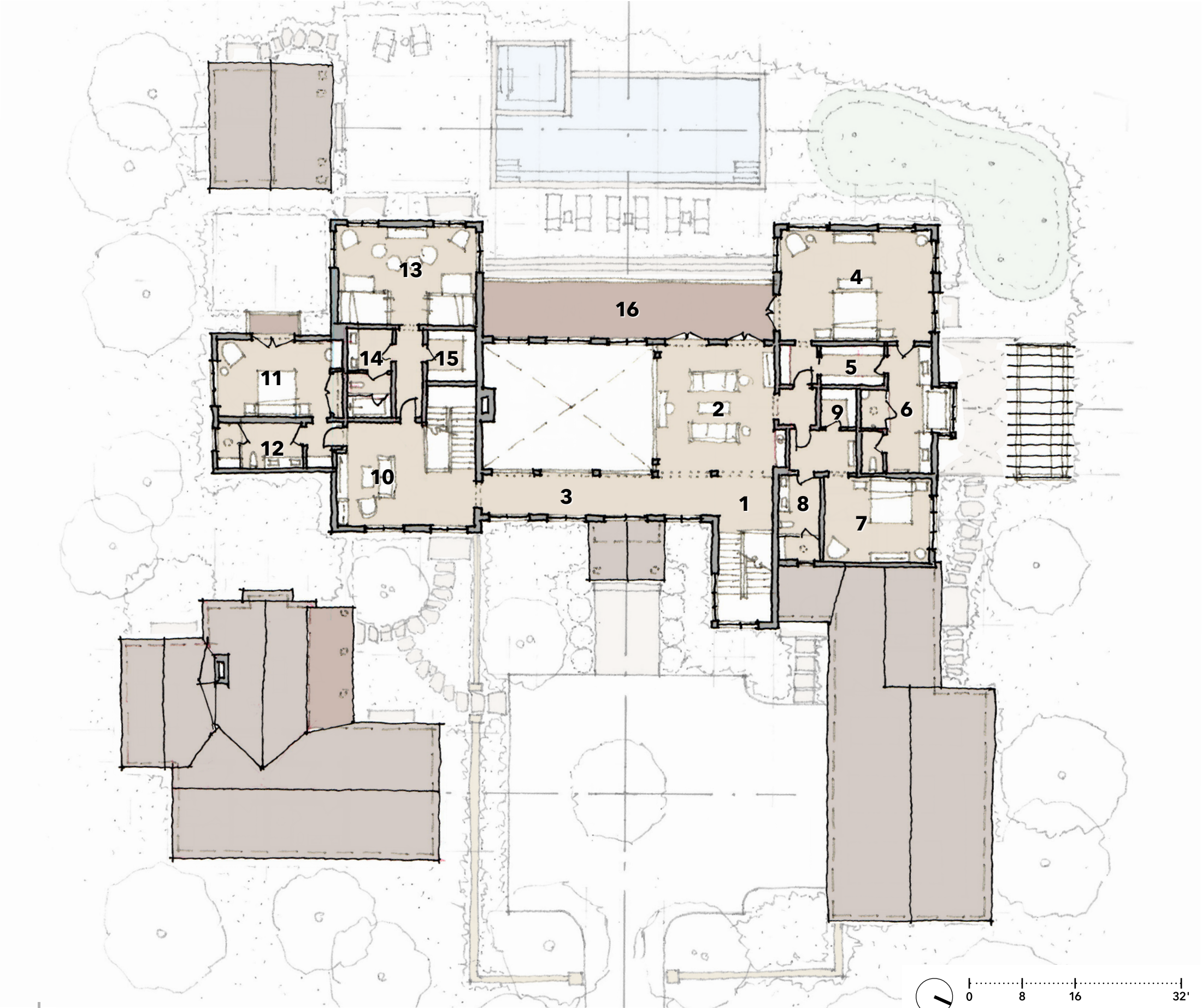
Woodland Estate Concept B | Upper Floor Plan
