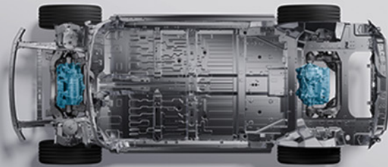
Front Double Wishbone + Independent Rear Five-link Suspension
