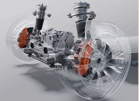
Akebono Front Four-piston Calipers
