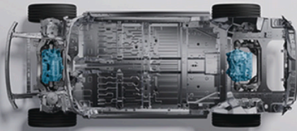
Front Double Wishbone + Independent Rear Five-link Suspension
