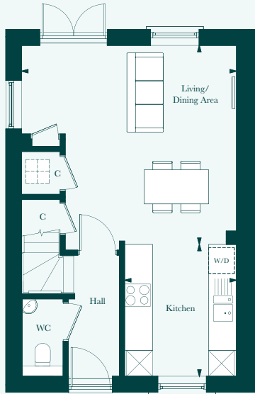
GROUND FLOOR Living Room/Dining 5m x 4.6m 16'6" x 15'2" Kitchen 2.6m x 3m 8'7" x 10'1"
