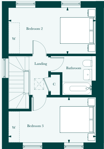
SECOND FLOOR Bedroom 2 5m x 2.6m 16'6" x 8'8" Bedroom 3 5m x 2.6m 16'6" x 8'6"
