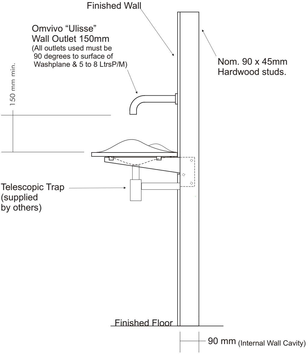
SIDE ELEVATION
