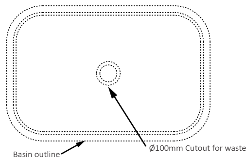
LATIS RECTANGULAR BASIN
