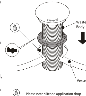
Figure 2. *Pop up plug and waste is indicative
