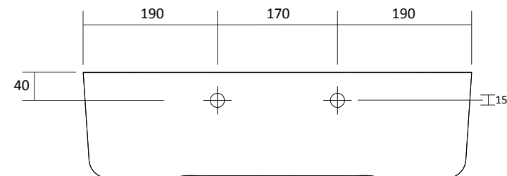
LILLI 550 WALL FIXING LOCATIONS
