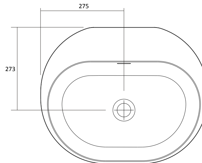
LILLI 550 WALL FIXING LOCATIONS
