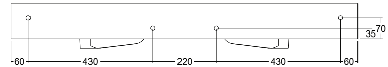
BACK VIEW
