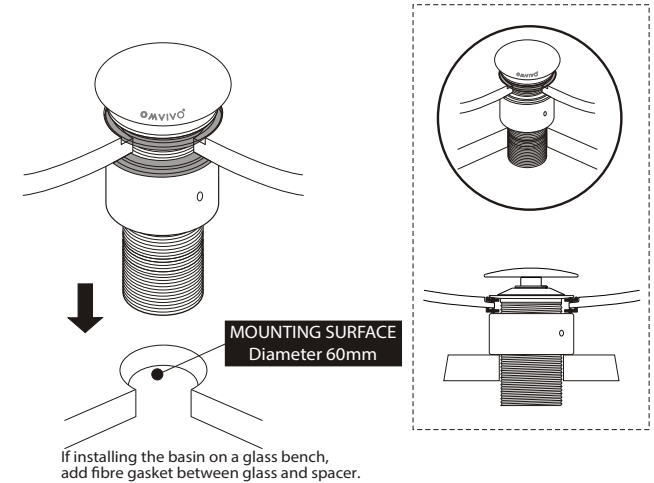
Figure 5. *Pop up plug and waste is indicative
