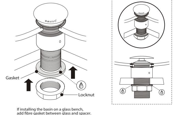
Figure 6. *Pop up plug and waste is indicative
