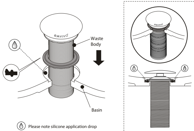
Figure 3. *Pop up plug and waste is indicative
