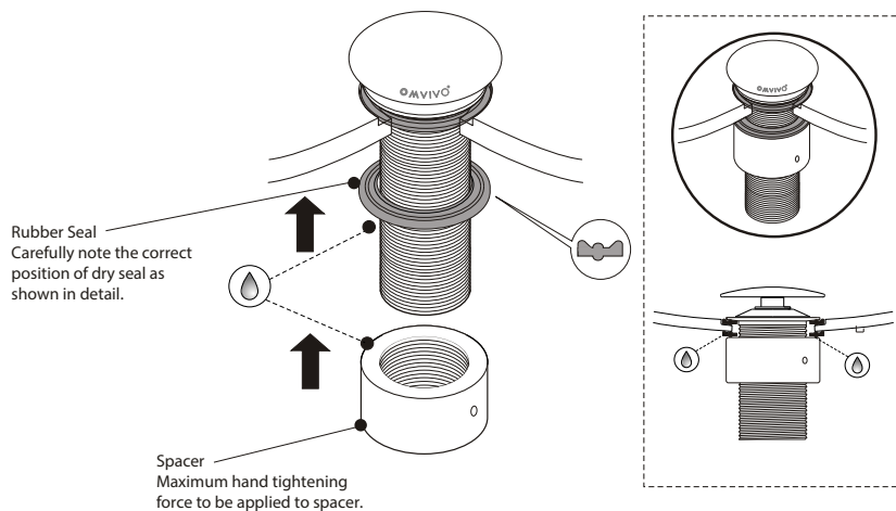
Figure 4. *Pop up plug and waste is indicative
