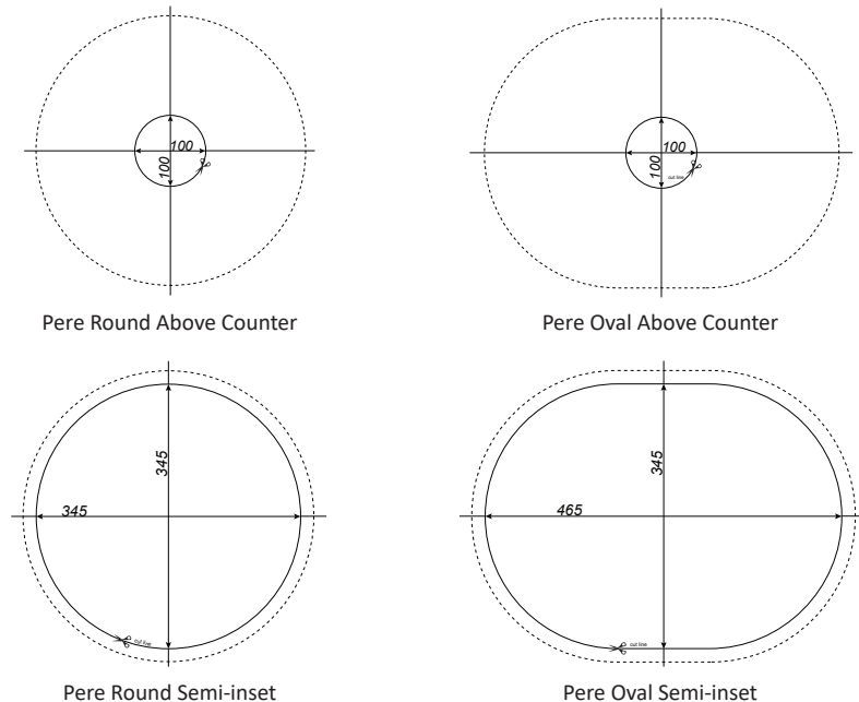
Figure 1. Pere basin bench top cut-out
