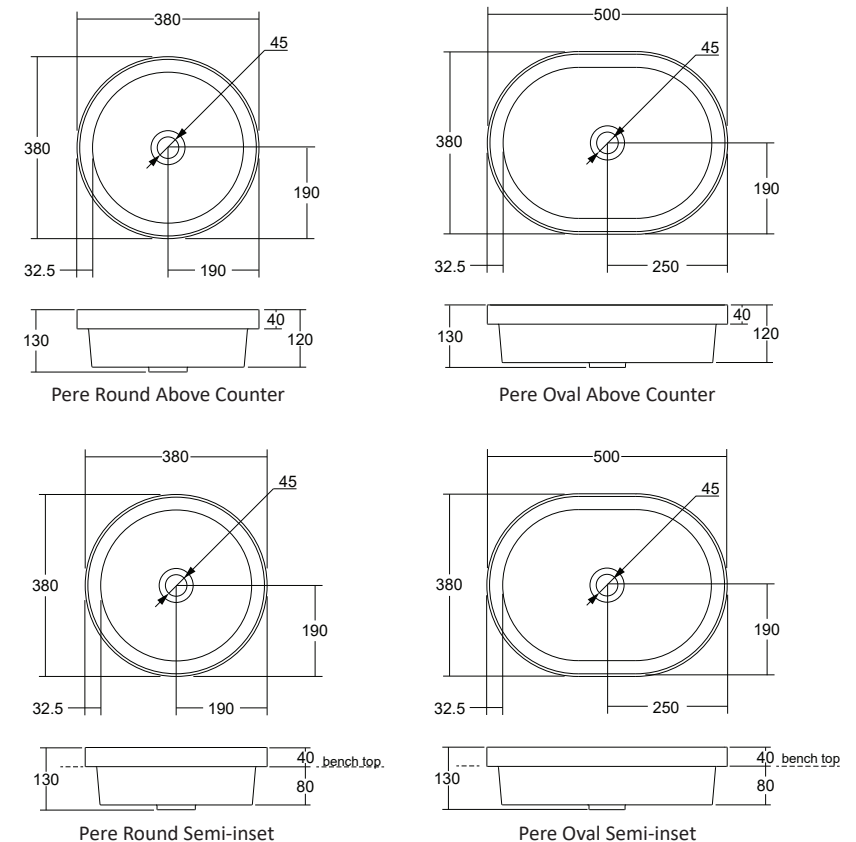
Figure 2. Pere basin product dimensions
