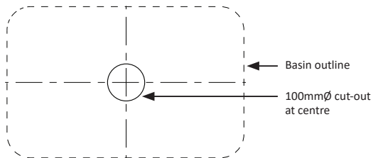
Figure 3. ABOVE COUNTER BASIN - PLACEMENT
