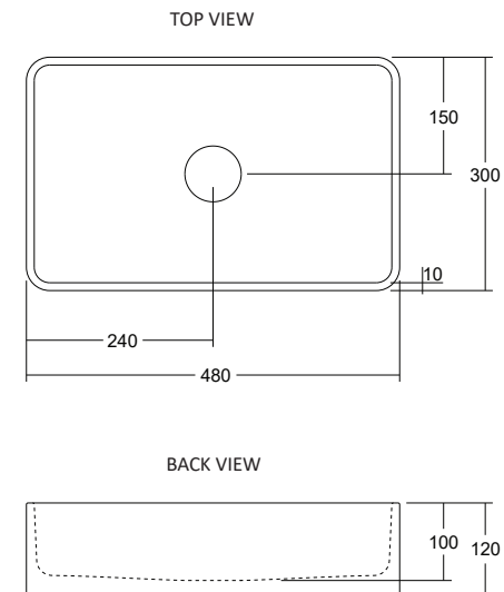
Figure 7. WASTE LOCATION MOD 480 ABOVE COUNTER BASIN
