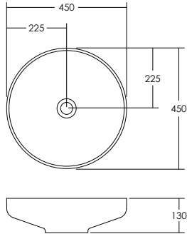
VENICE 450 ROUND BASIN
