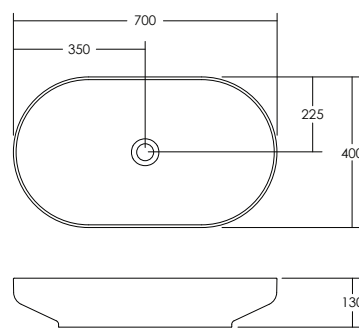
VENICE 700 OVAL BASIN
