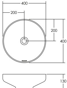
VENICE 400 ROUND OVERFLOW BASIN
