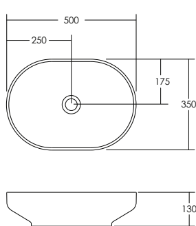
VENICE 500 OVAL BASIN
