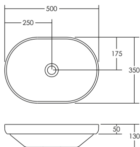
VENICE 500 OVAL SEMI-INSET BASIN
