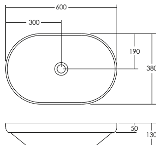
VENICE 600 OVAL SEMI-INSET BASIN
