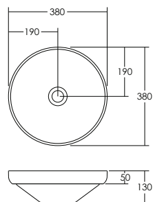
VENICE 380 ROUND SEMI-INSET BASIN
