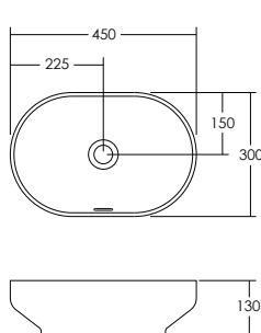
VENICE 450 OVAL OVERFLOW BASIN
