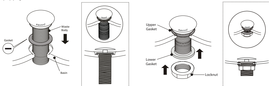
Figure 5. Waste assembly detail *Pop up plug and waste is indicative
