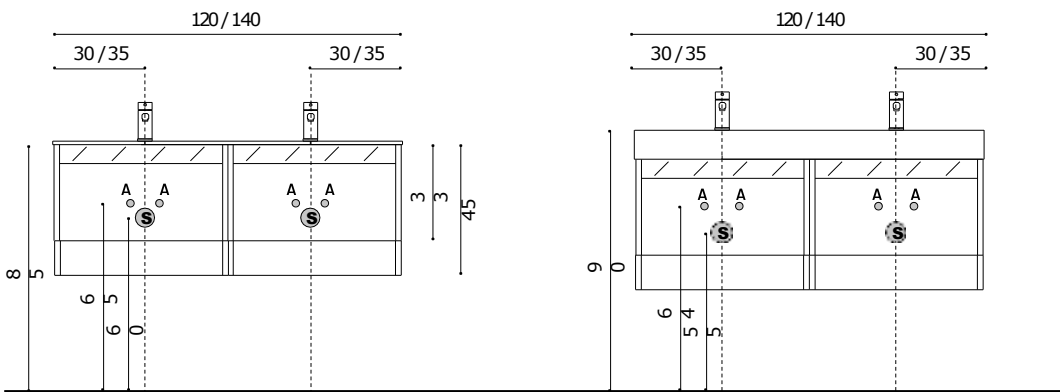
QUOTE BASI PORTALAVABO 2 VASCHE CON LAVABO INTEGRALE QUOTAS DISCHARGES BASE UNIT FOR INTEGRAL WASHBASIN
