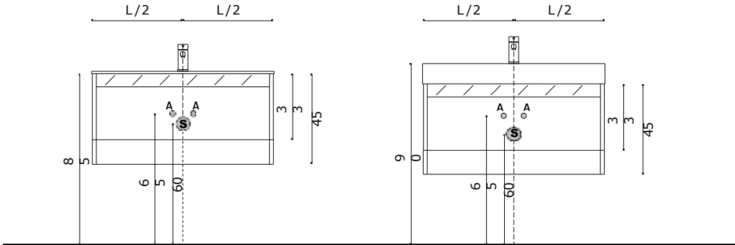
QUOTE BASI PORTALAVABO CX CON LAVABO INTEGRALE QUOTAS DISCHARGES BASE UNIT FOR INTEGRAL WASHBASIN CX
