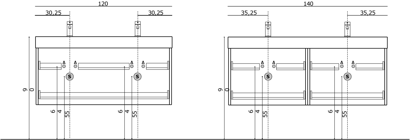
QUOTE BASI PORTALAVABO DOPPIA VASCA CON LAVABO SHARK H.10 (ES. FIANCHI H.50) QUOTAS DISCHARGES BASE UNIT FOR WASHBASIN WITH DOUBLE BASIN WASHBASIN SHARK H.10 (EX. SIDES H.50)
