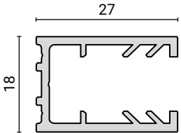
PROFILO A MURO WALL PROFILE WANDPROFIL PROFIL MURAL
