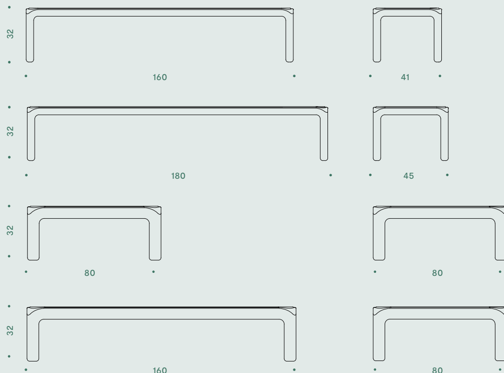
VISTA FRONTAL FRONT VIEW VISTA FRONTALE
