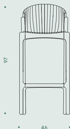
VISTA FRONTAL FRONT VIEW VISTA FRONTALE
