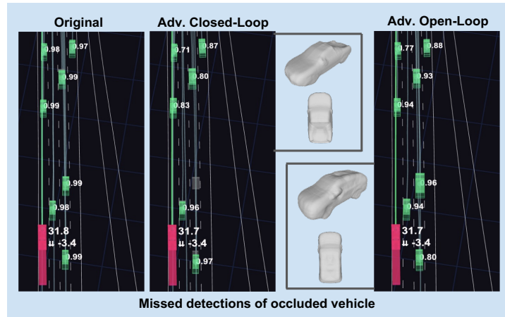
Figure A8: Qualitative examples of adversarial shape generation in closed loop vs open loop. ADV3D is able to generate adversarial actors that cause detection failures due to occlusion but the open-loop counterpart fails.
