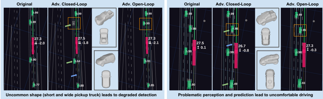
Figure 4: Qualitative examples of adversarial shape generation in closed loop vs open loop. We highlight the modified actors using orange bboxes and show generated adversarial shapes aside. The perception and prediction failures are pointed out by green and blue arrows. Specifically, the green arrows point to the green detected bounding boxes, and blue arrows point to the predicted light blue trajectories. The numbers on top of green predicted bounding boxes are the detection confidence scores. The numbers beside the pink ego-truck denote the current velocity and acceleration.
