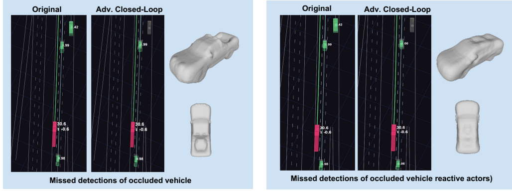
Figure A7: Qualitative examples of adversarial shape generation (non-reactive actors vs reactive actors). ADV3D is able to generate adversarial actors that cause detection failures due to occlusion.
