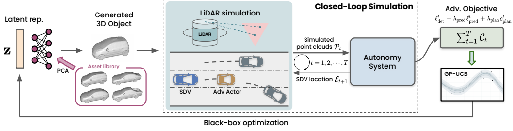
Figure 2: Overview of ADV3D for safety-critical 3D object generation in closed-loop. Given a real-world scenario, Adv3D modifies the shapes of selected actors, and runs LiDAR simulation and full autonomy stack in closed-loop to optimize the shape representation with black-box optimization.
