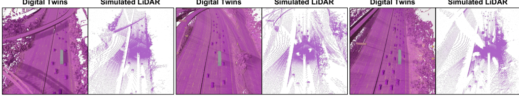
Figure 3: Reconstructed digital twins and simulated LiDAR for real-world highway scenarios.
