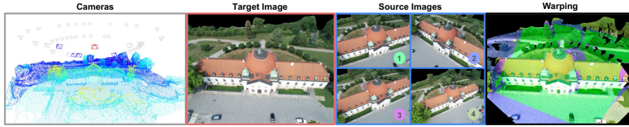
Fig. A1: Large view changes on BlendedMVS. We highlight the target view in red and 4 closest source views in blue. The distance and view-orientation changes between the source views and the target view are large. The image warping (rightmost column, colored by image source index, missing regions in black) shows that limited source views cannot get full coverage to synthesize the target view.
