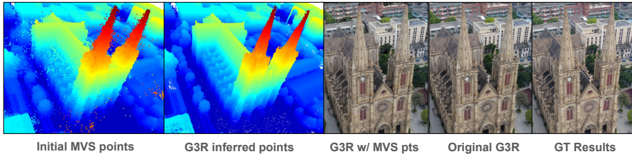
Fig. A12: G3R is robust to point initialization (zoom-in).
