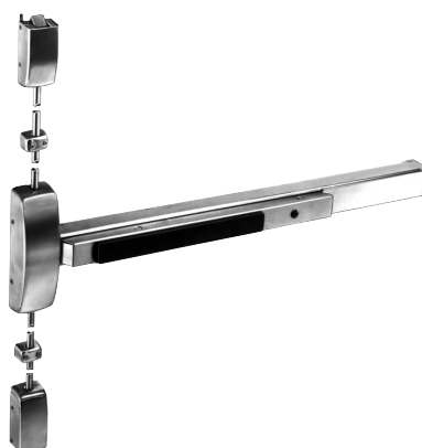
8700 Surface Vertical Rod
