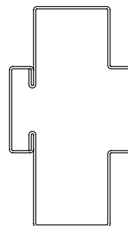
2 Piece Mullion
