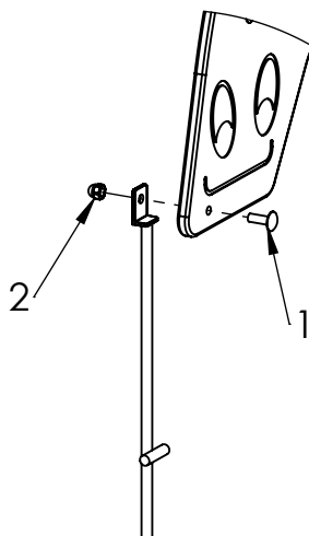
DETAIL D SCALE 1 : 10
