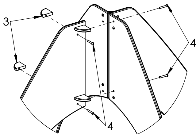
DETAIL A SCALE 1 : 13
