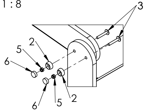
DETAIL E SCALE 1 : 8
