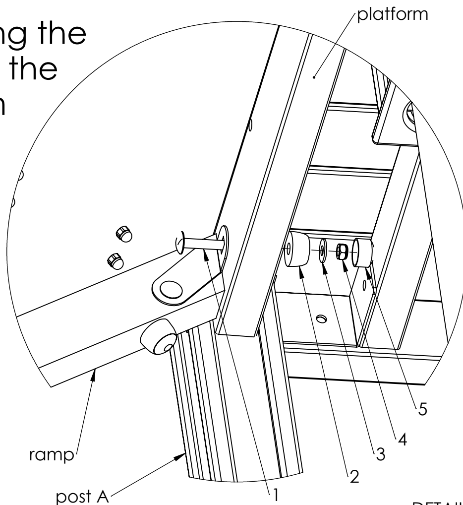
DETAIL K
