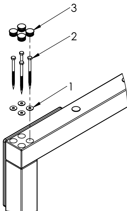
DETAIL A SCALE 1 : 10
