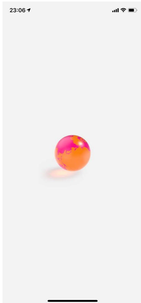
1 - Open App
