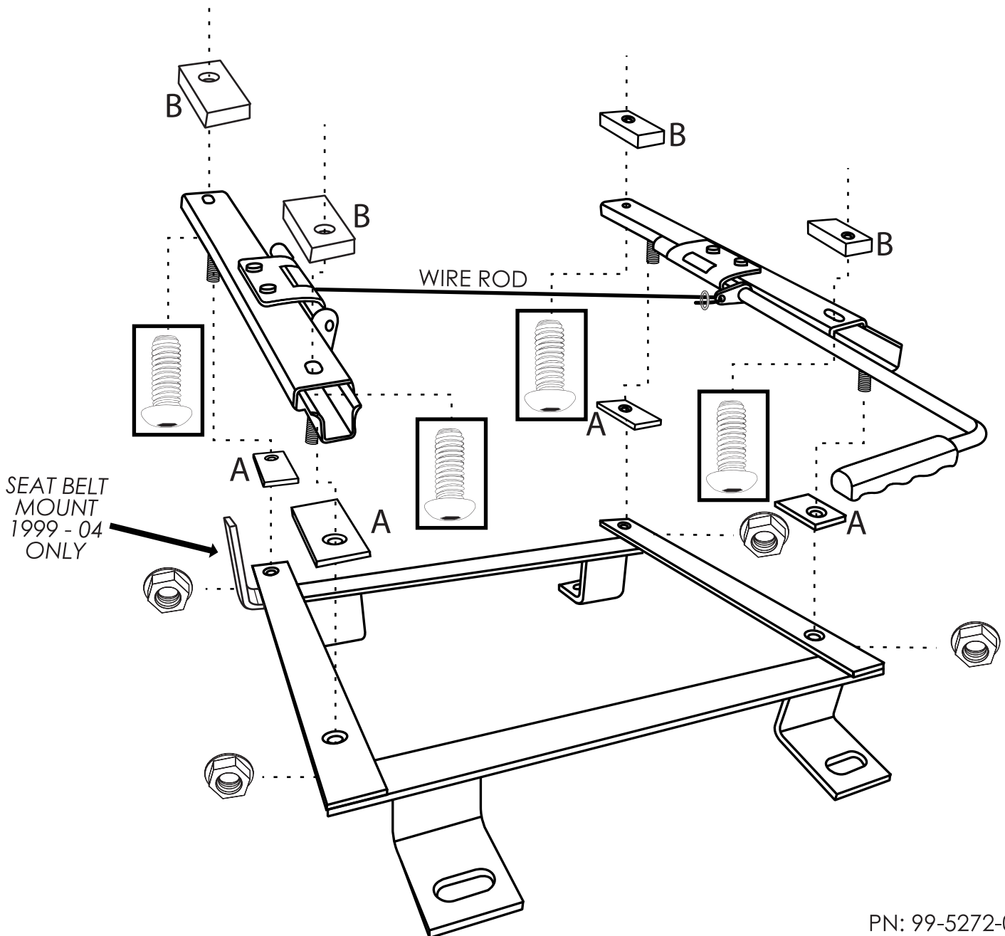
Flat Style Bracket (2) Brackets fit Right or Left
