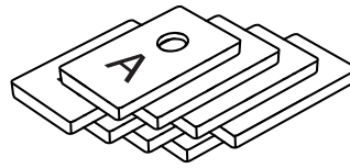
(8) Bracket Slider Spacers (A) 3/16" X 2" X 1"
