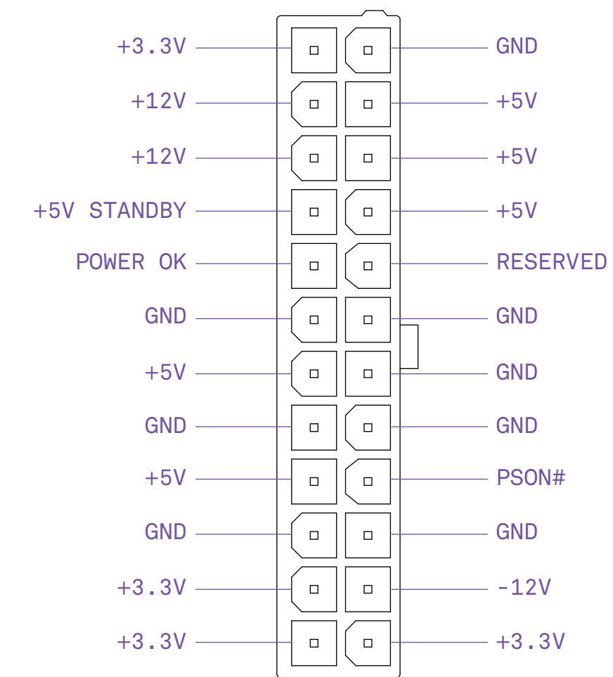
24-pin ATX_POWER
