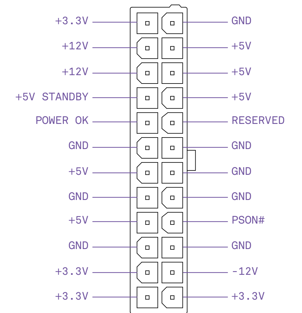
24-pin ATX_POWER
