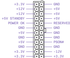
24-pin ATX POWER
