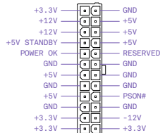
24-pin ATX_POWER
