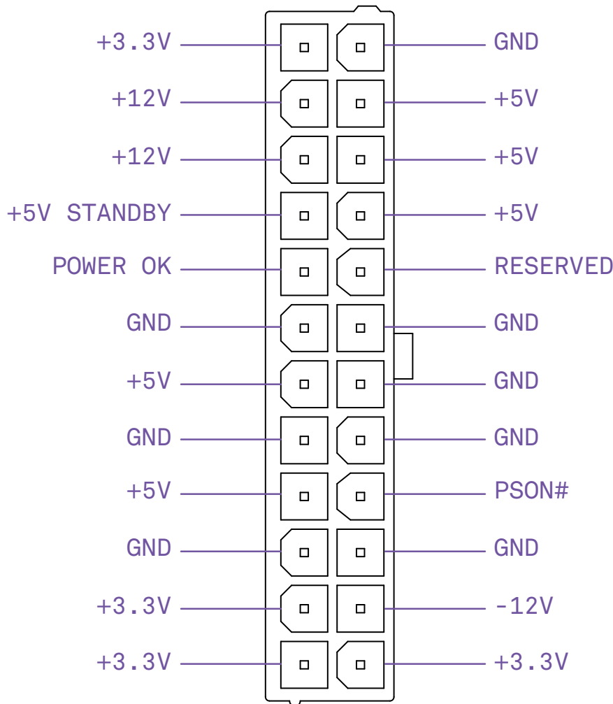
24-pin ATX_POWER
