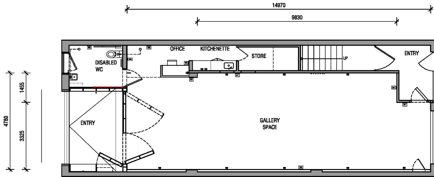
GLASSHOUSE GALLERY PLAN 1:100@A4
